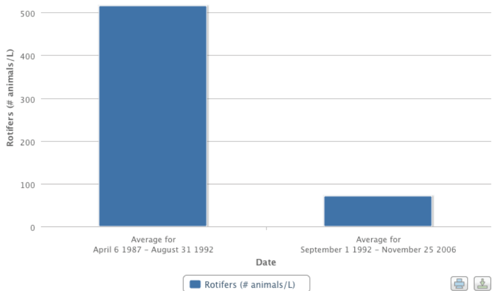
This bar graph shows the change in the average number of rotifers per liter (micro-zooplankton) at the Kingston station before and after zebra mussels became established in 1992.
