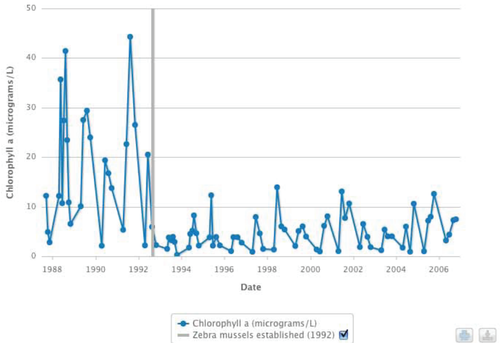
This graph shows the change in concentration of Chlorophyll a (representing phytoplankton biomass) between 1988 and 2006 at the Kingston station. The gray line indicates the date that zebra mussels first became established in the river.
