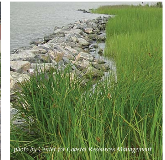
A vertical wall (left) offers poorer habitat than a riprapped revetment (center) or sill and wetland (right), and also reflects waves.
